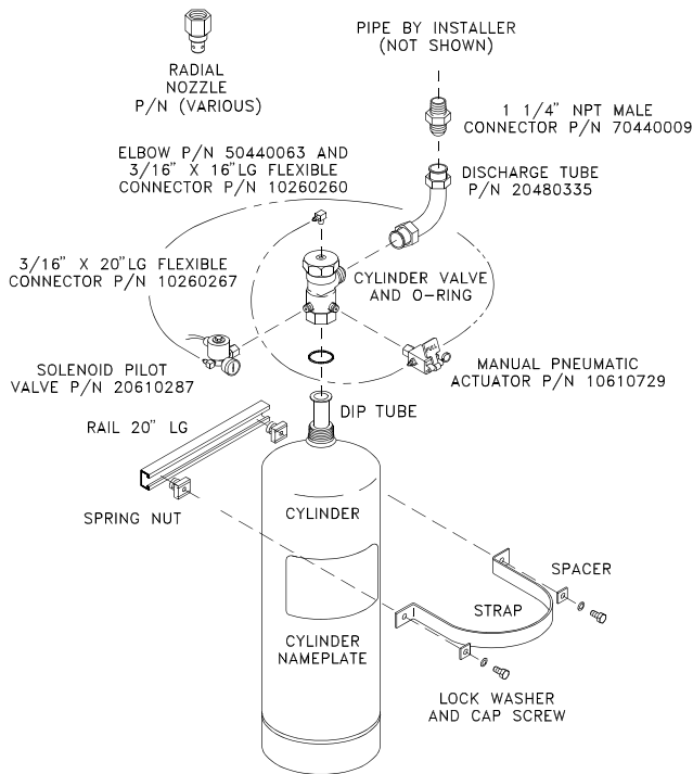
Beta Series Cylinder Assembly with Completer Kit, Mounting Bracket & Nozle
