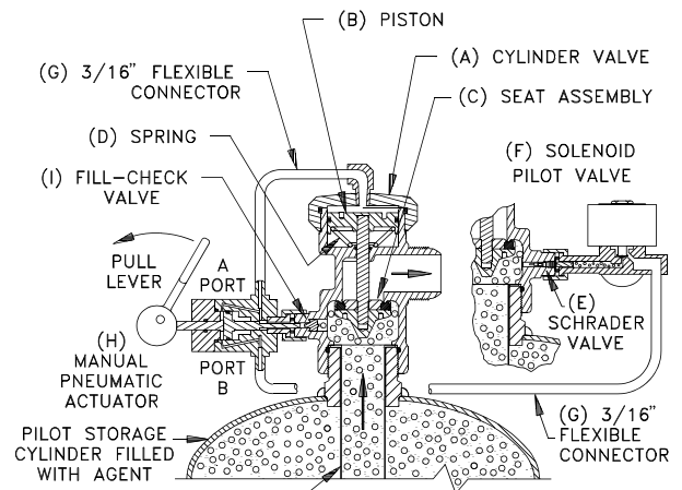
Cylinder Valve -Standby Mode
