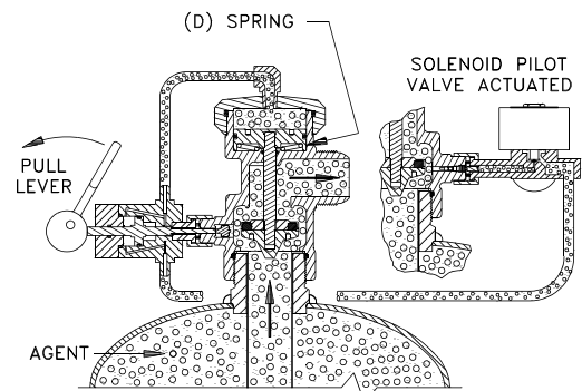
Cylinder Valve -Actuated Mode
